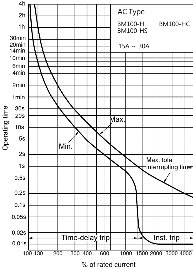
Operating Characteristics
