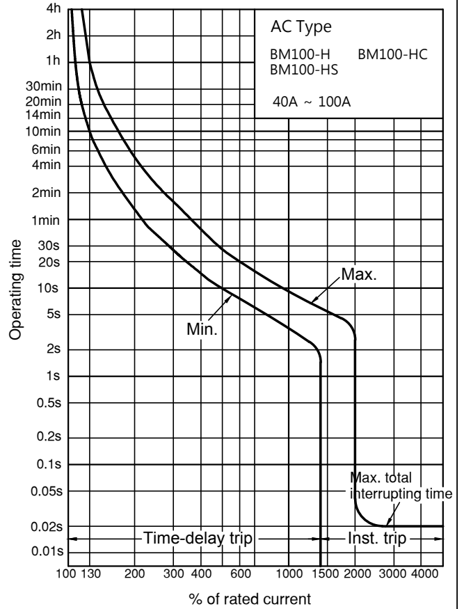
Operating Characteristics
