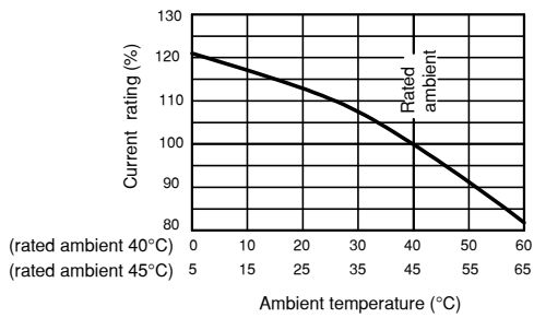
Compensation Curve
