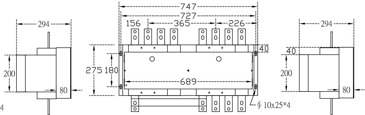
4P, 630AF/800AF
