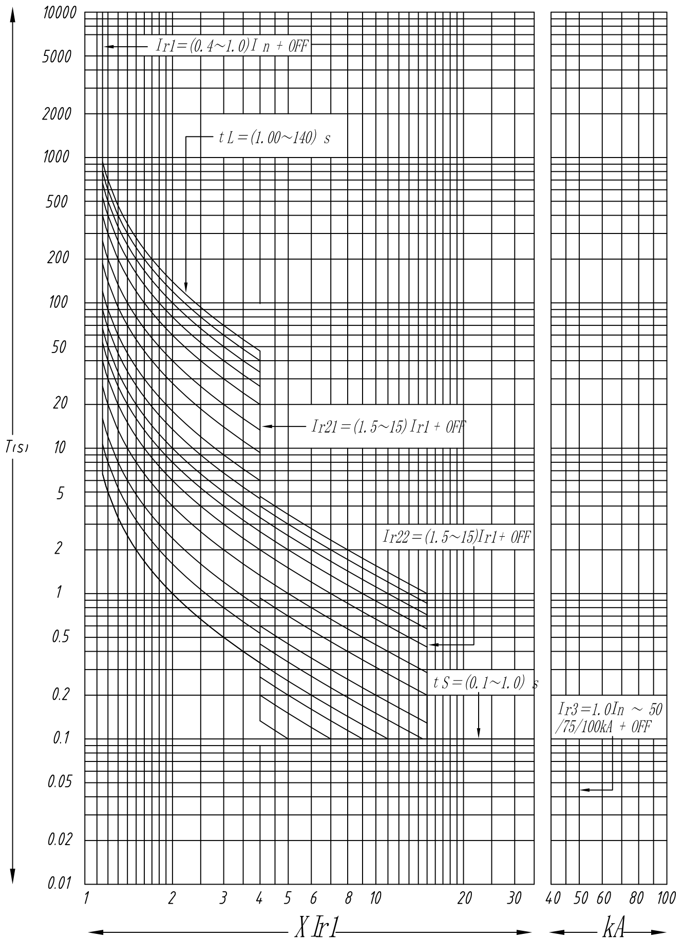
Curve 2 : Quick inverse time
