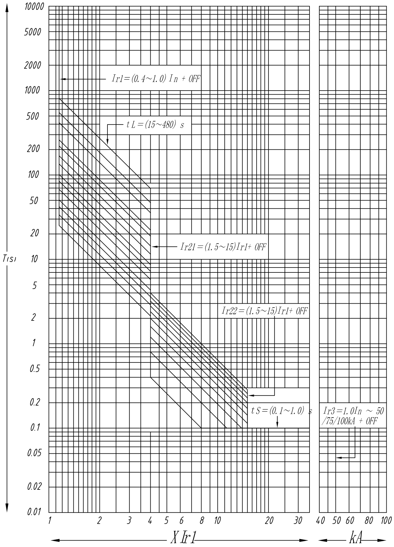
Curve 6 : Super inverse time 2 (General purpose)
