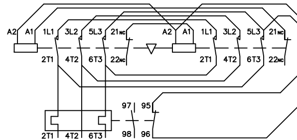
Circuit diagram
