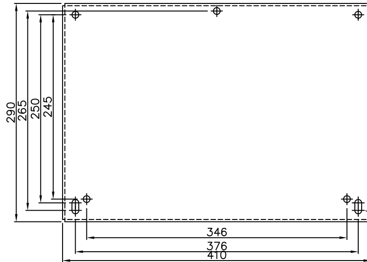
Mounting holes for M8 screws (7 places)
