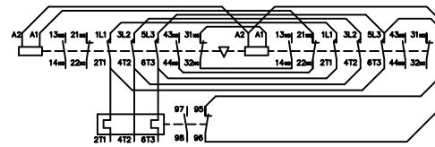
Circuit diagram
