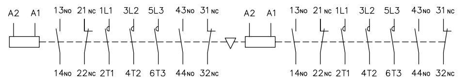
Circuit diagram
