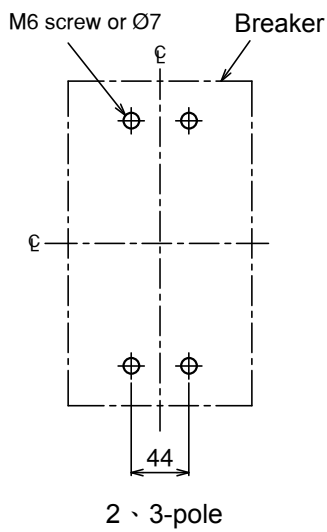
Drilling plan
