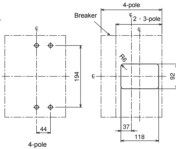
Drilling plan
