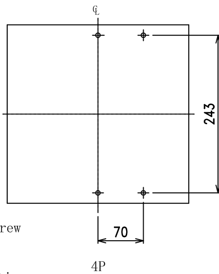
Mounting
