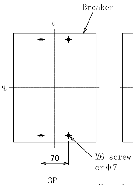
Mounting
