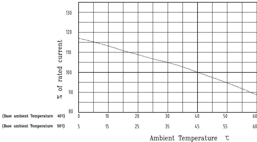
Compensation Curve
