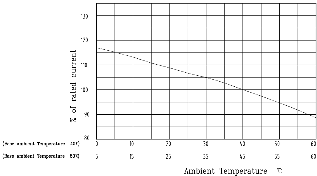
Compensation Curve
