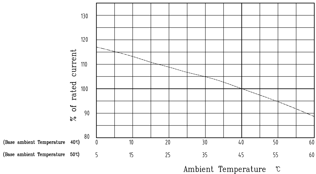
Compensation Curve
