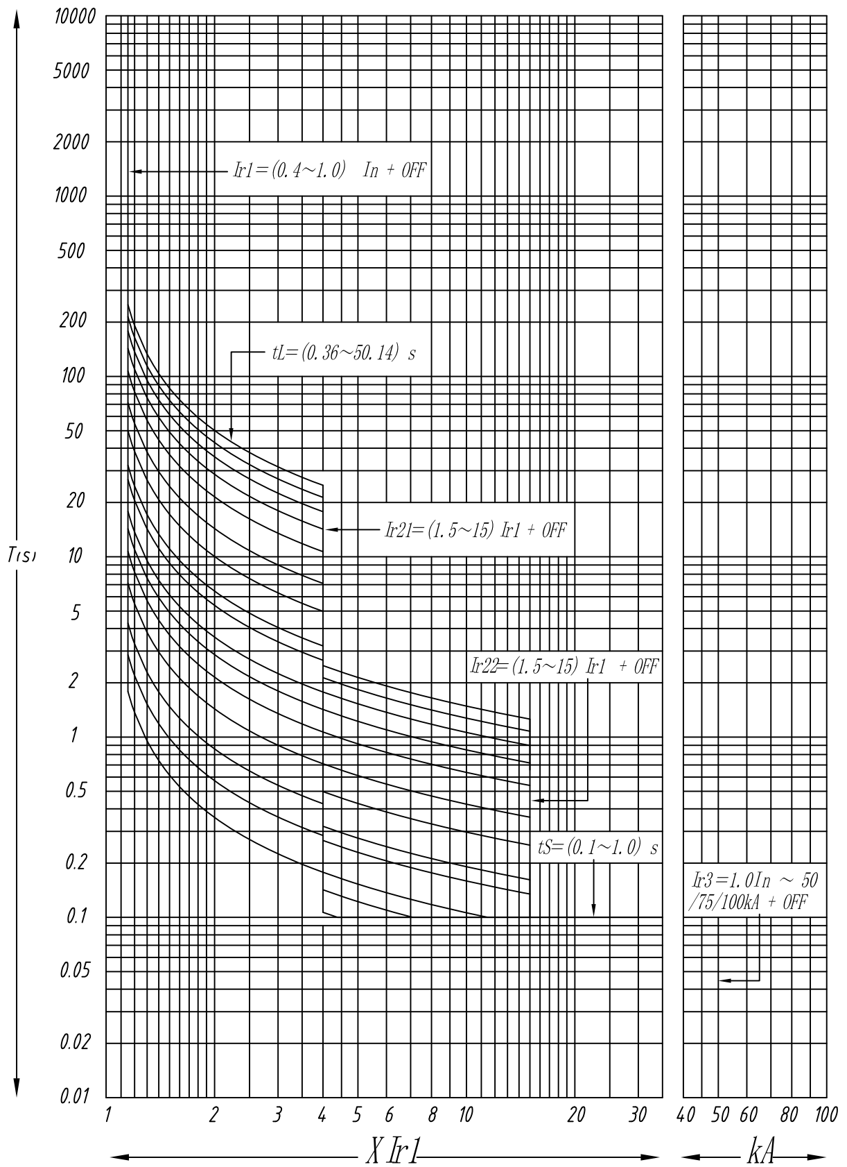
Curve 1 : Standard inverse time
