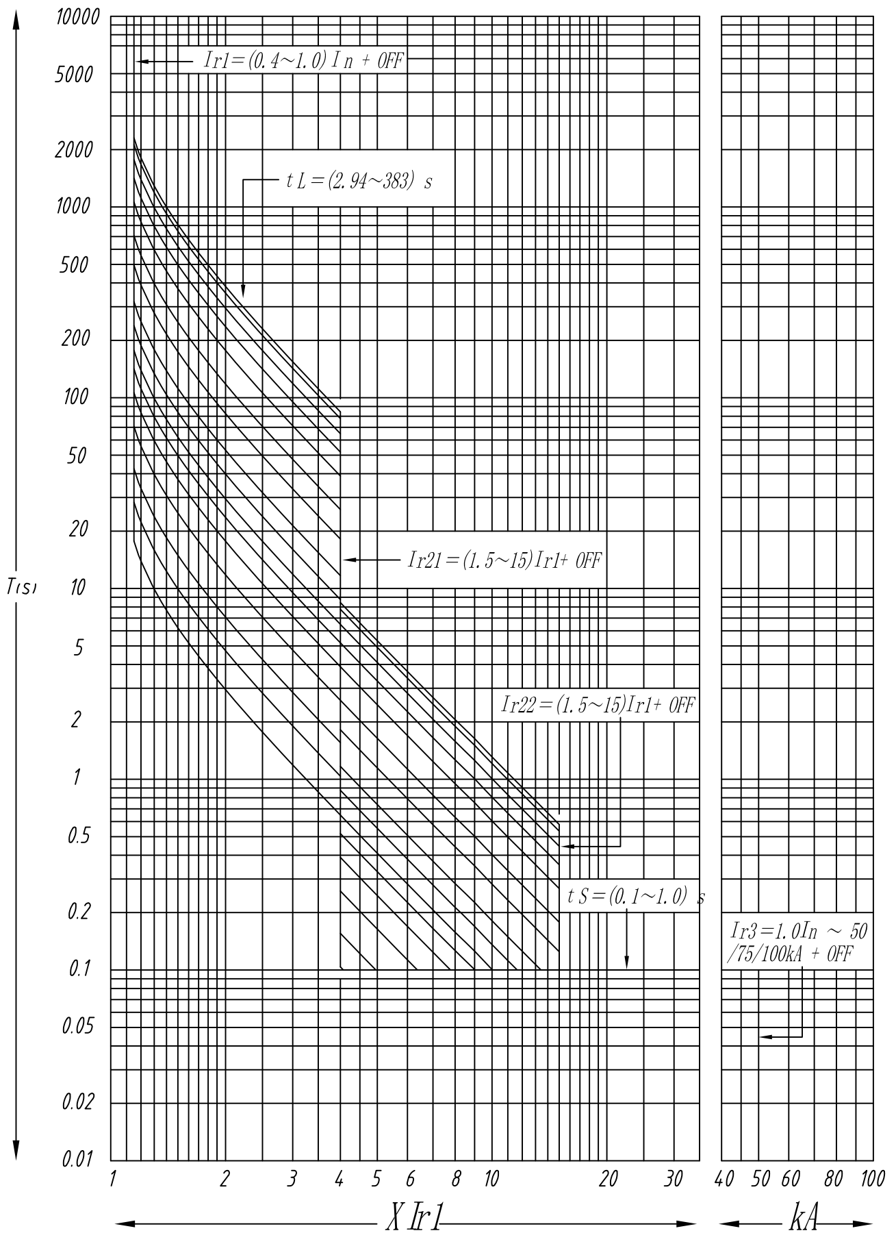
Curve 4 : Super inverse time (Motor protection)
