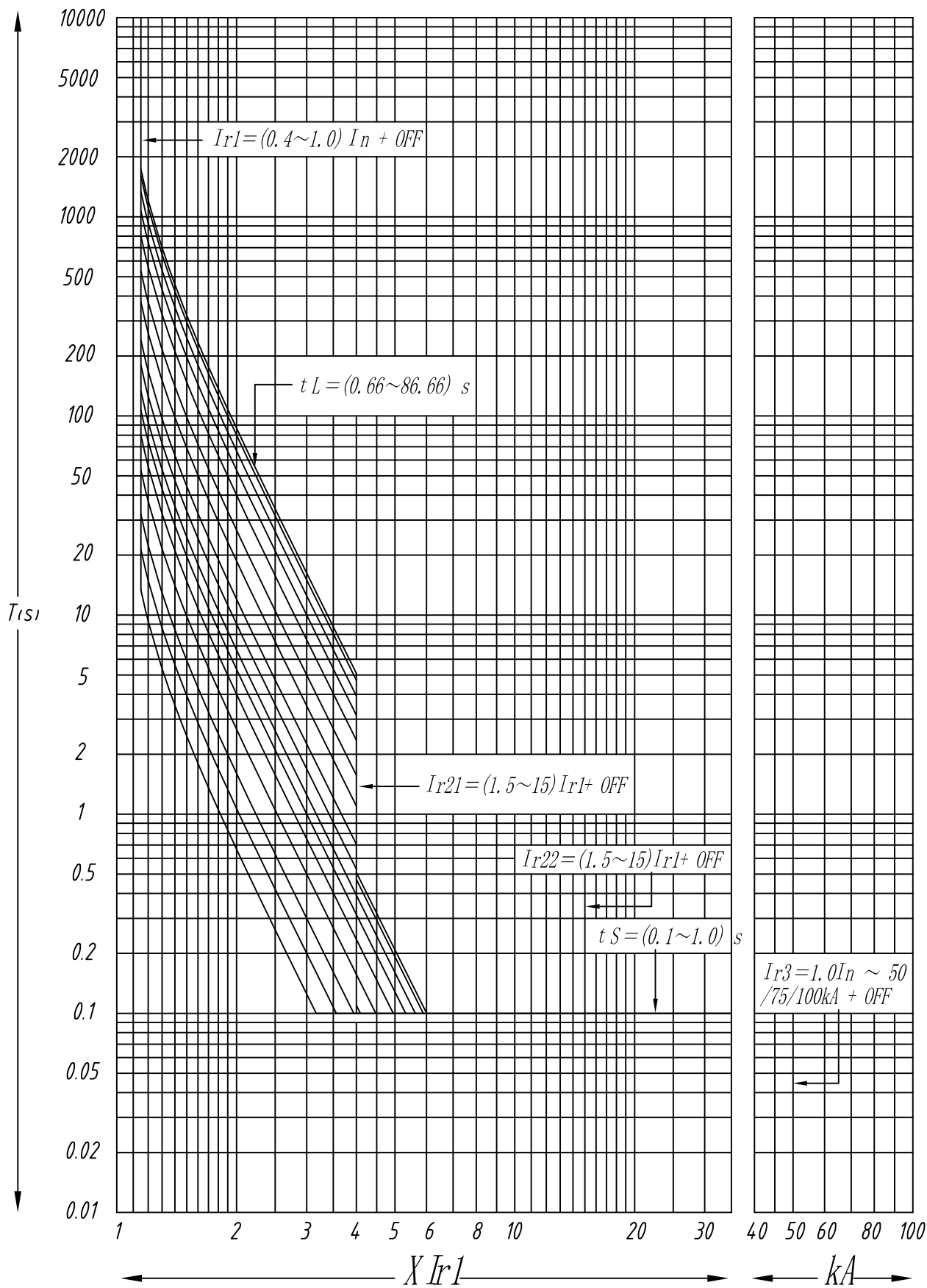
Curve 5 : High-voltage fuse compatibility
