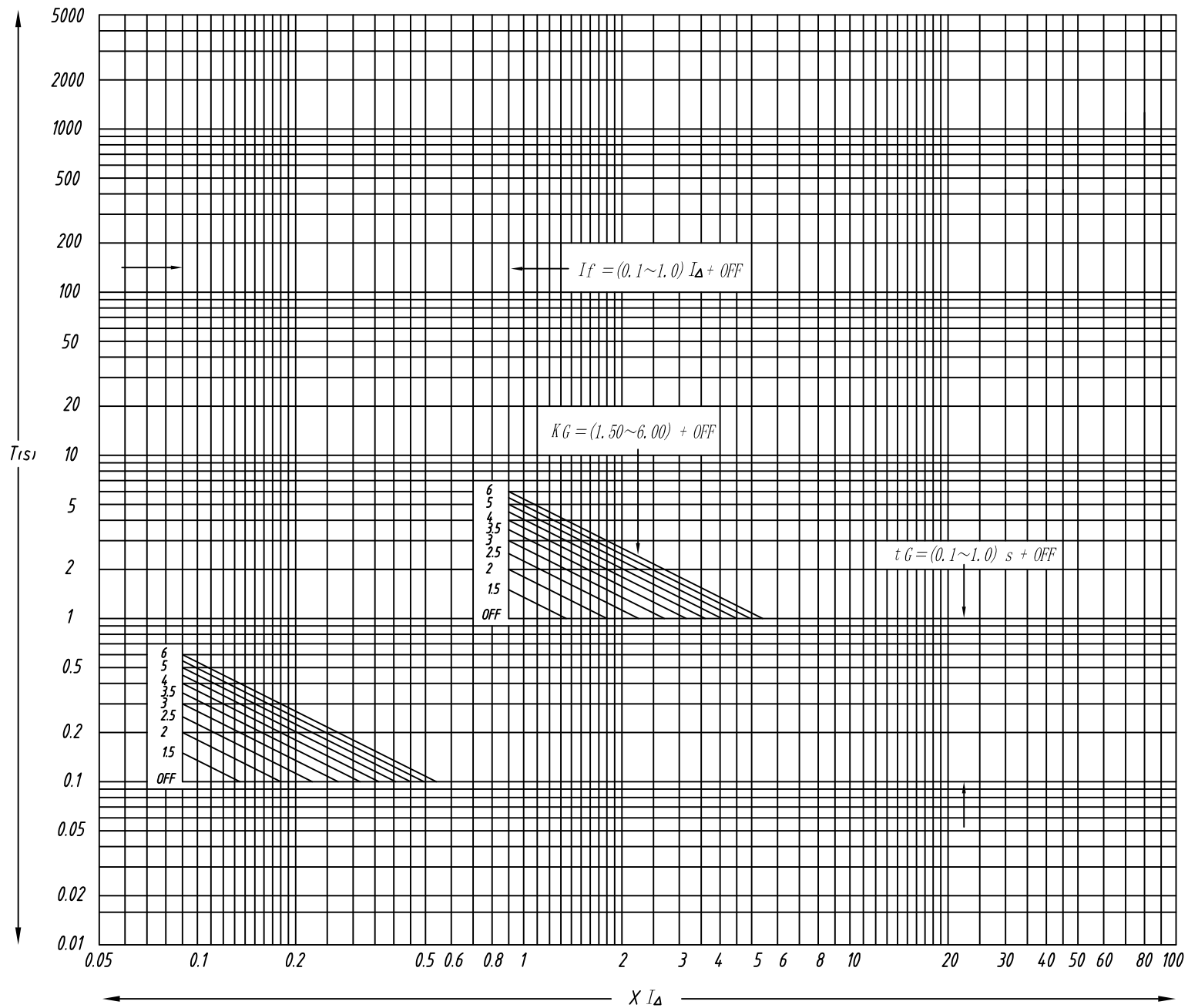
Leakage characteristic curve (External transformer mode)
