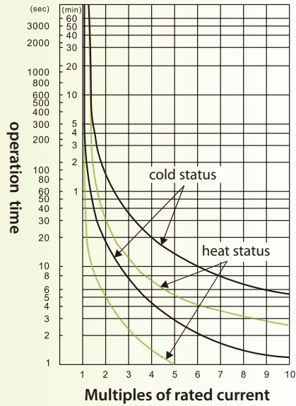
TH-P18ES – below 6.5A tripping characteristic curve
