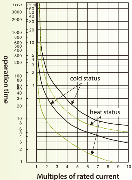
TH-P20ES TA – above 9A tripping characteristic curve
