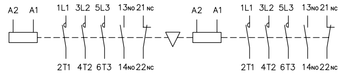
Circuit diagram
