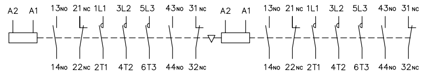
Circuit diagram
