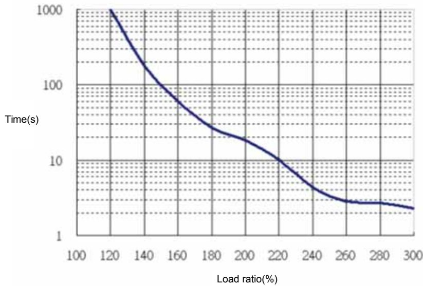
SMA-L050/L100 overload protection curve
