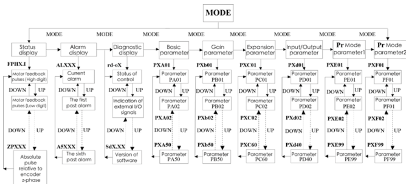
Chart 1: Display flowchart
