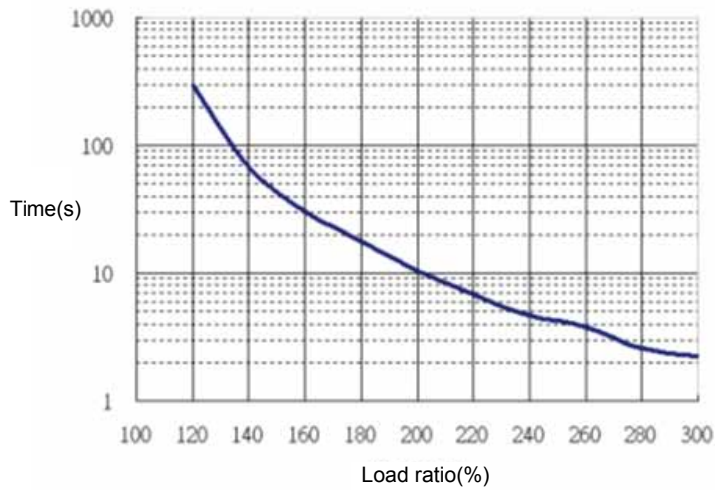
SMA-L020-L075 overload protection curve
