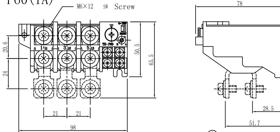
Installation Dimension
