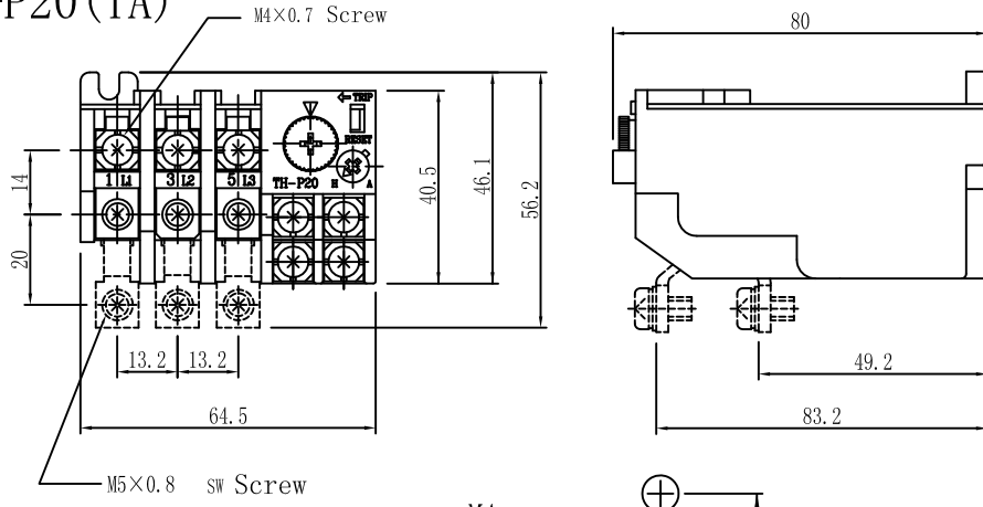
Installation Dimension
