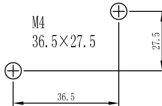
Installation Dimension
