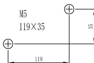
Installation Dimension
