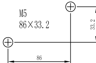
Installation Dimension
