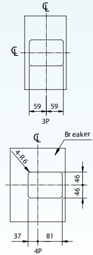
Panel cut
