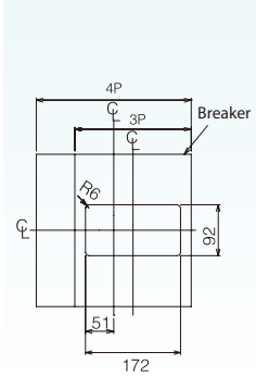
Panel cut
